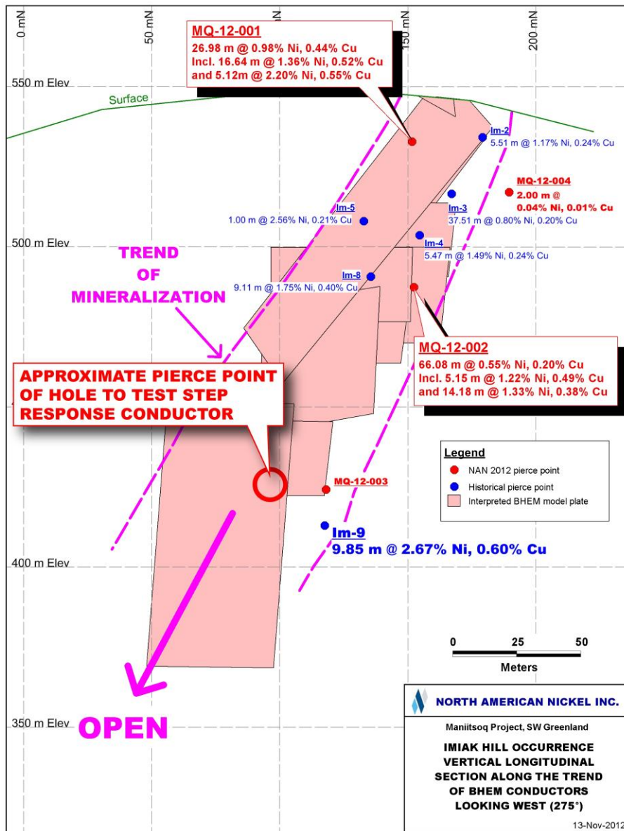
Figure 3: Vertical longitudinal section along the Imiak Hill mineralized zone looking west showing the approximate pierce point of a proposed hole to test the off hole step response EM conductor detected from hole MQ-12-003.
